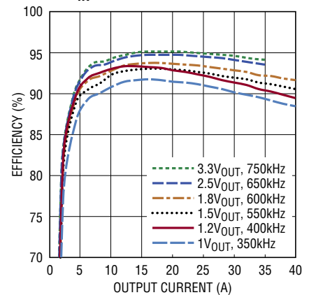
Efficiency vs Load Current with 12\text{V}_{IN}
