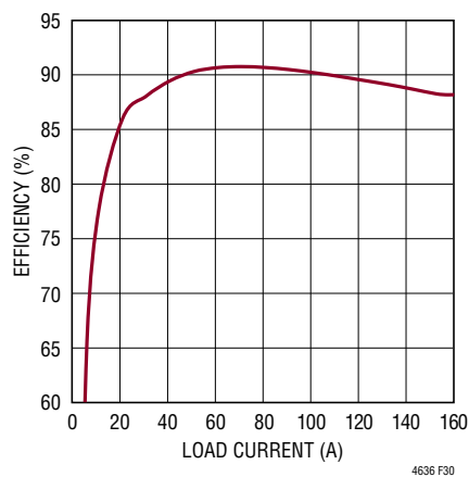
Figure 30. Efficiency, 12V to 0.9V at 160A
