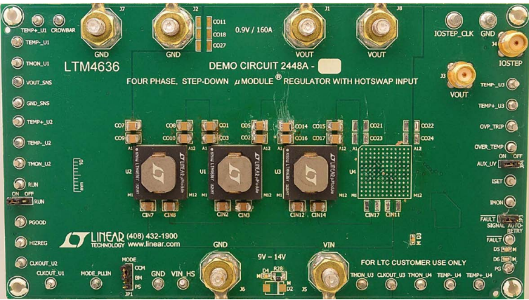
Figure 23. Demo Board
