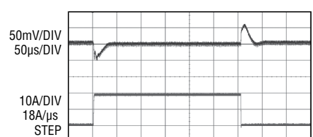
1.2V Transient Response
