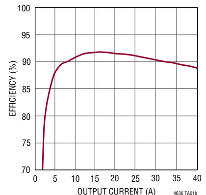
12V IN , 1V OUT Efficiency vs Output Current
