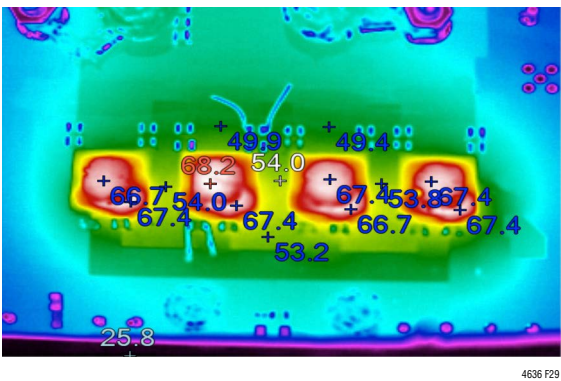
Figure 29. Thermal Plot, 12V to 0.9V at 160A, 400LFM Air Flow
