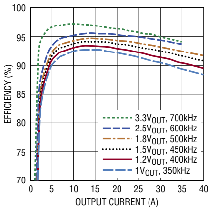
Efficiency vs Load Current with 8\text{V}_{IN}
