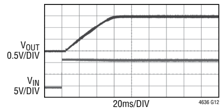
Start-Up with Soft-Start Full Load
