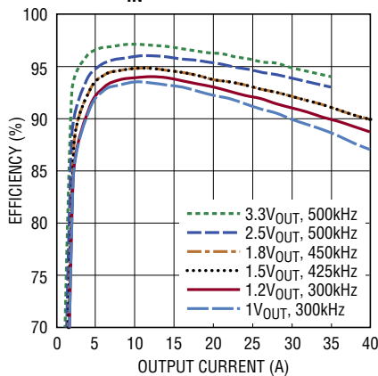
Efficiency vs Load Current with 5\text{V}_{IN}
